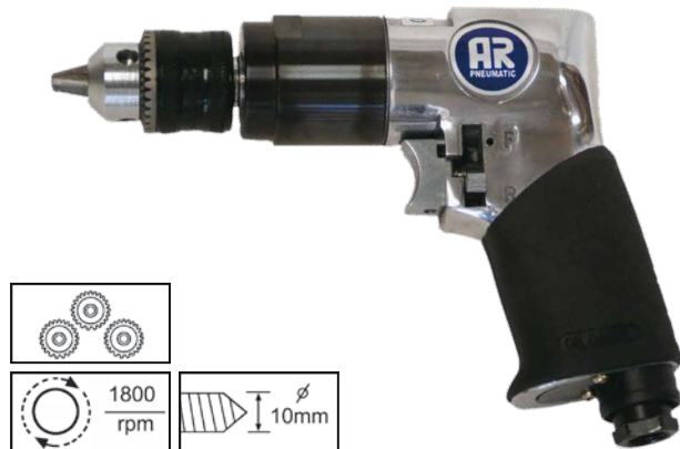
AR-3002 TALADRO REVERSIBLE 3/8"
