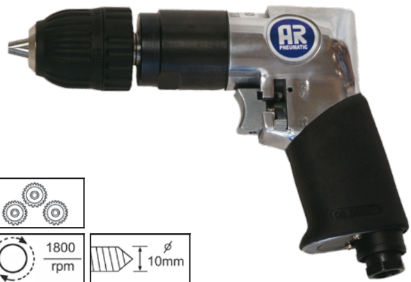
AR-3002B TALADRO REV. 3/8" PORTABROCAS AUTOM.
